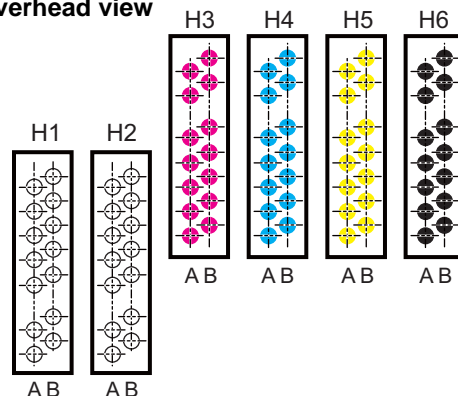
Nozzle pattern
